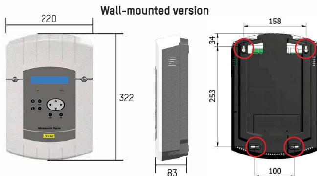
Mounting holes
